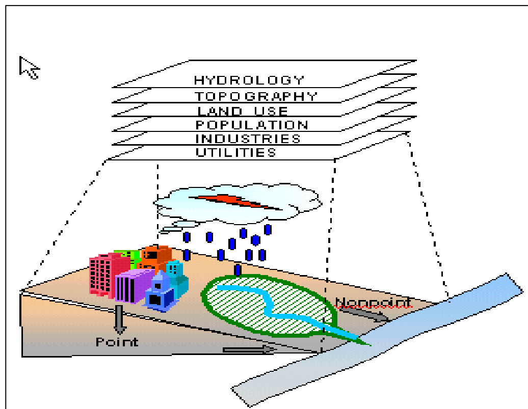
Figure 17-2. Factors influencing load model
