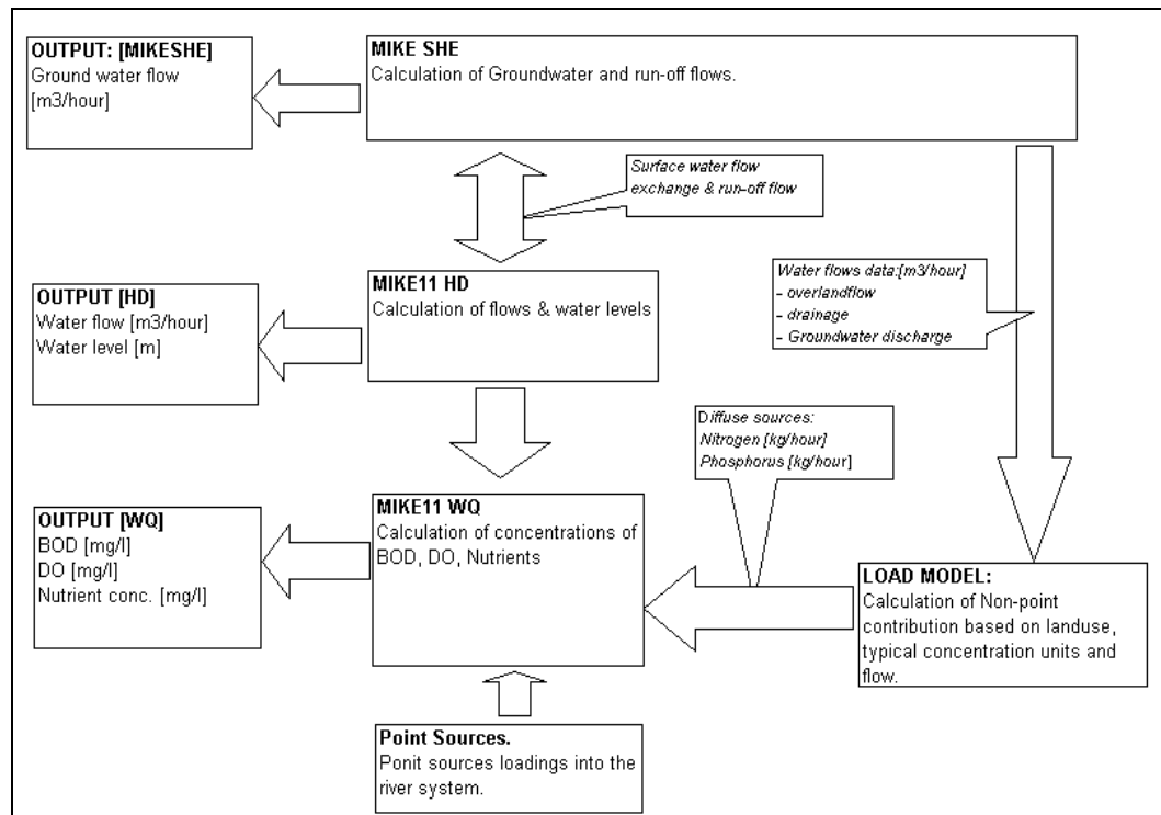
Figure 17-1. The Integrated Model Set-Up
