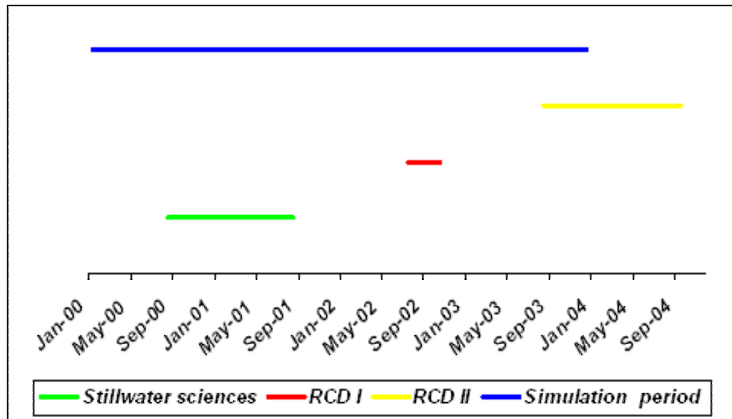
Figure 17-5. Monitoring Data Coverage from the Three Monitoring Campaigns and the Suggested Simulation Period
