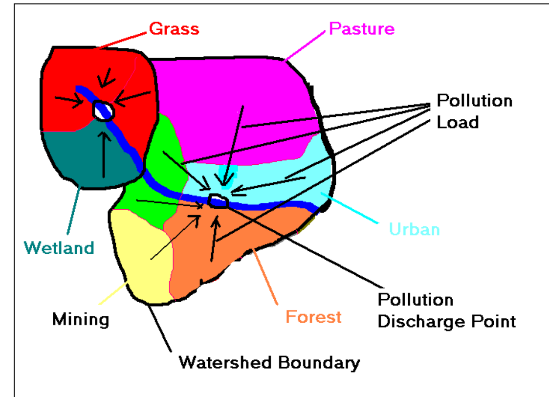
Figure 17-3. Principal of the Load Calculations
