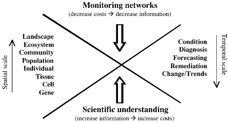
Figure 1 Illustration of the suite of ecological indicators ( left ) for which a suite of assessment capabilities ( right ) are desired. Constraints on the development of ecological indicators at all levels for all assessment endpoints are due to a lack of scientific understanding and the predominance of policies requiring low cost monitoring. Goals in applications generally include a compromise between cost-effectiveness and the ability to defend the ecological indicator scientifically at the spatial and temporal scale appropriate to answer the desired management objectives.
