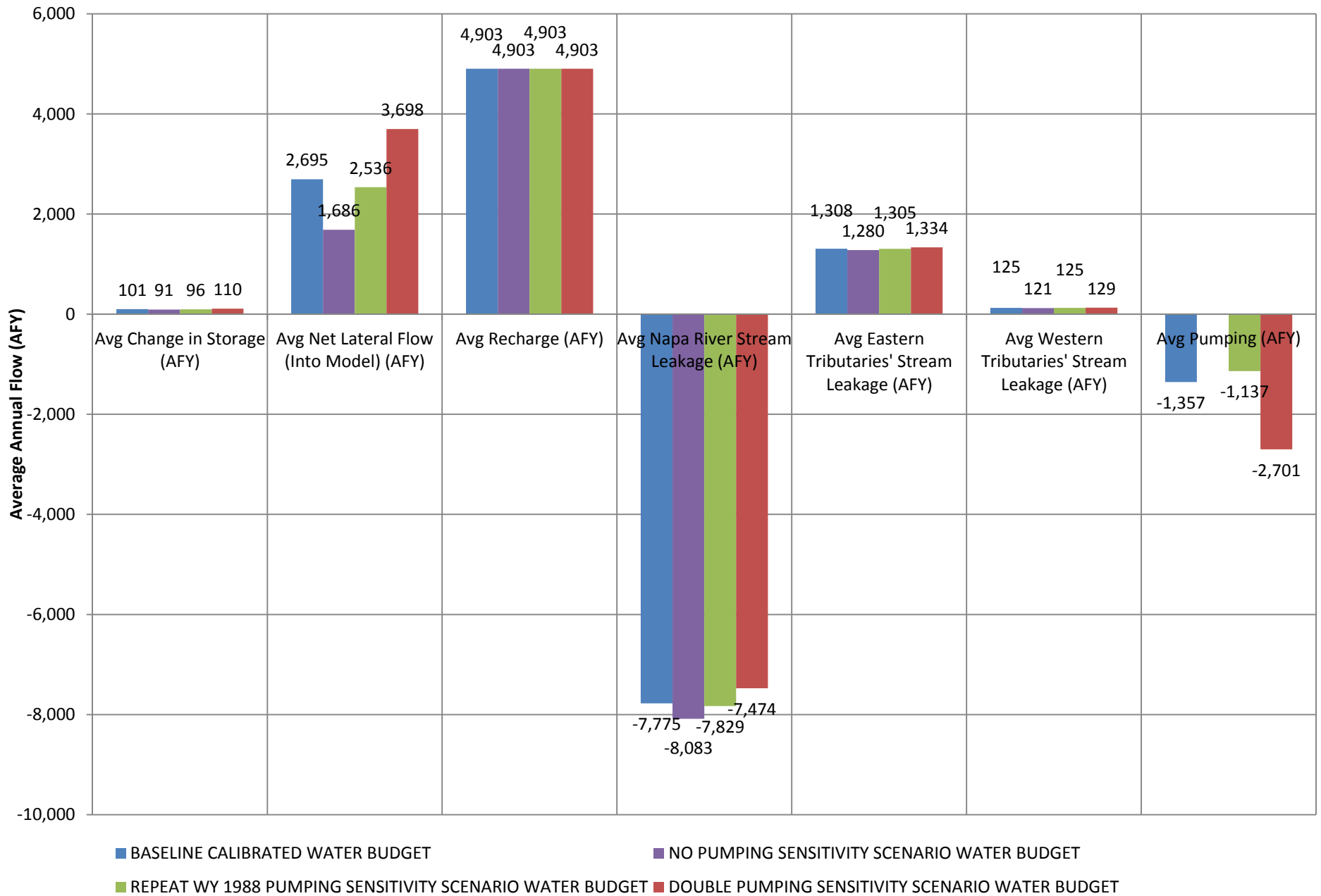
FIGURE 3-30 Average Annual Water Budget Components for Baseline and Three Pumping Sensitivity Scenarios Northeast Napa Area: Special Groundwater Study
