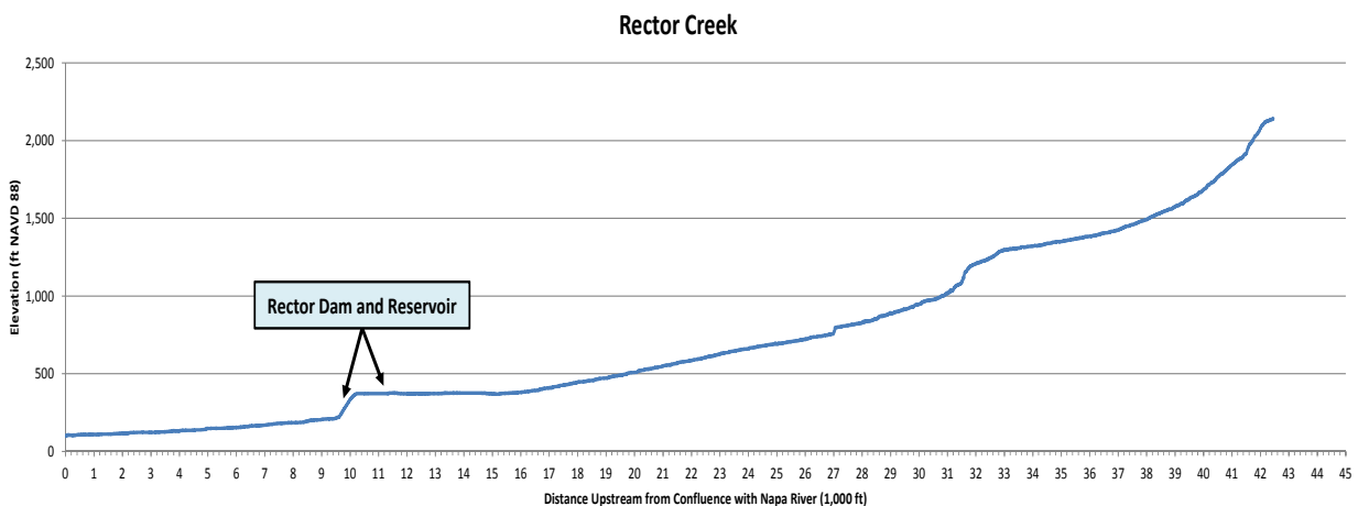
Figure 7-6. Estimated Stream Thalweg Elevations for Rector Creek
