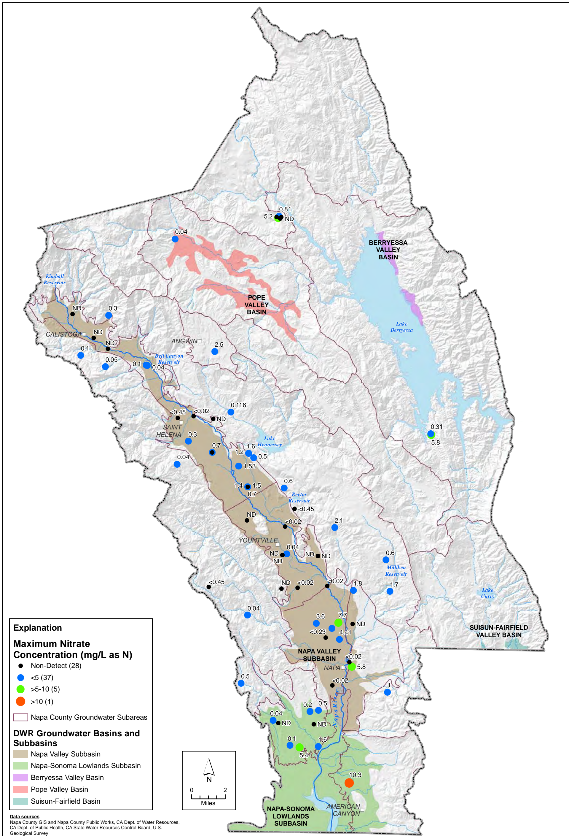
FIGURE 6-5 Maximum Nitrate Concentrations in Groundwater, 2009 - 2015 Napa County, CA
