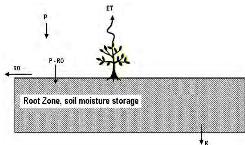
Figure ES-3. Conceptual Diagram of the Water Balance within the Root Zone
