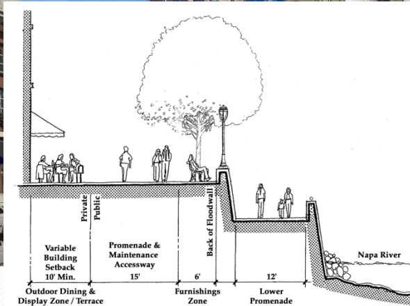
Floodwall Trail / Promenade Sta. 770+00
