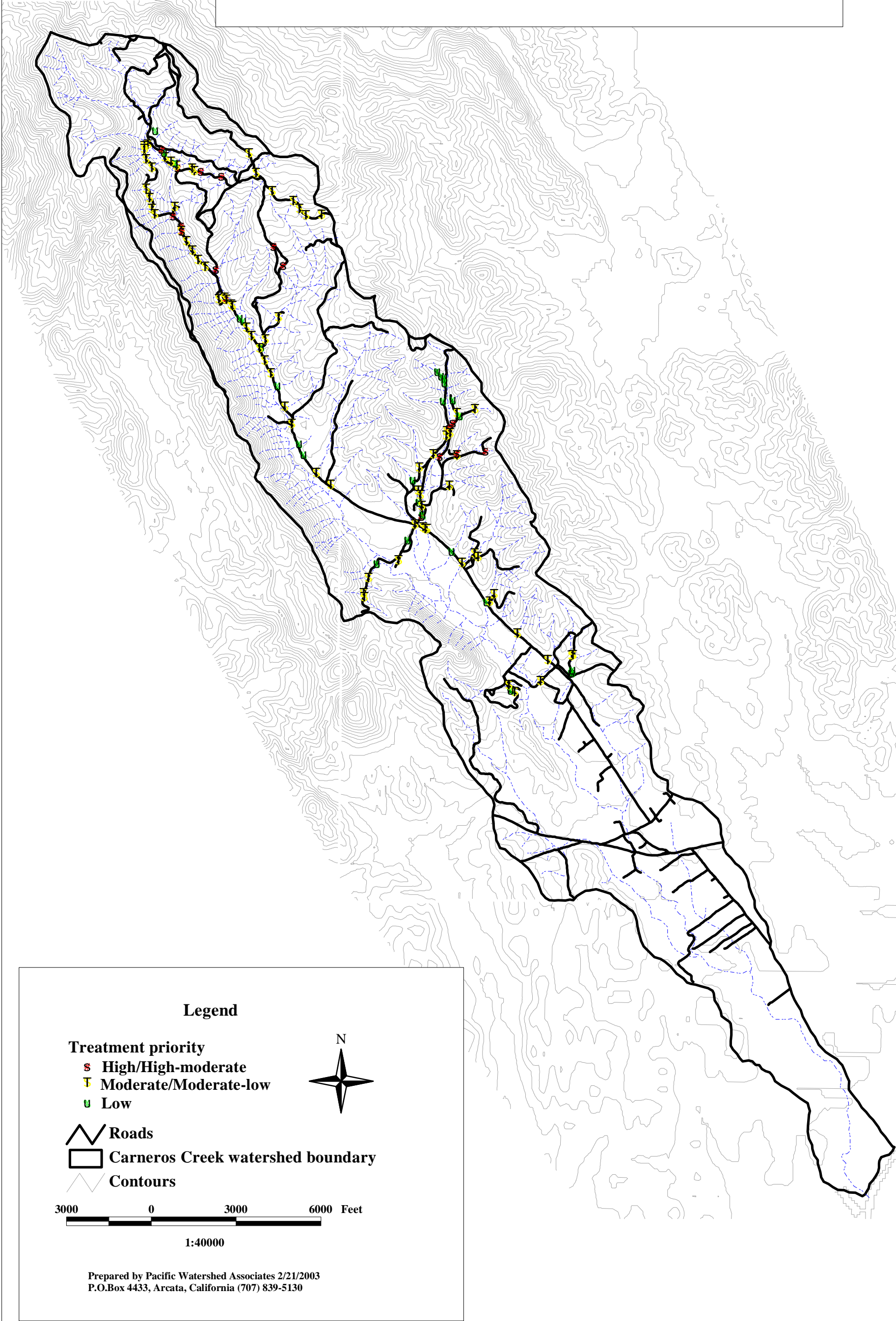
Map 7. Road-related sites with future sediment delivery by treatment priority, Carneros Creek, Napa County, California
