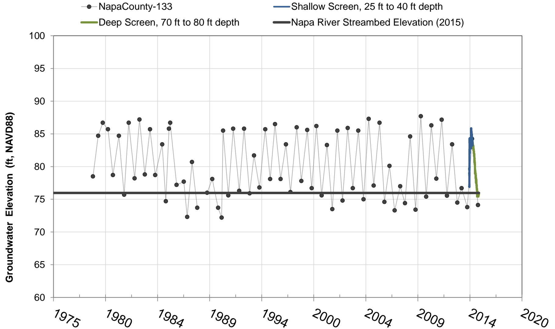
Figure 4-47 Surface Water-Groundwater Network Site Historical Comparison Site 4: Napa River at Yountville Cross Road
