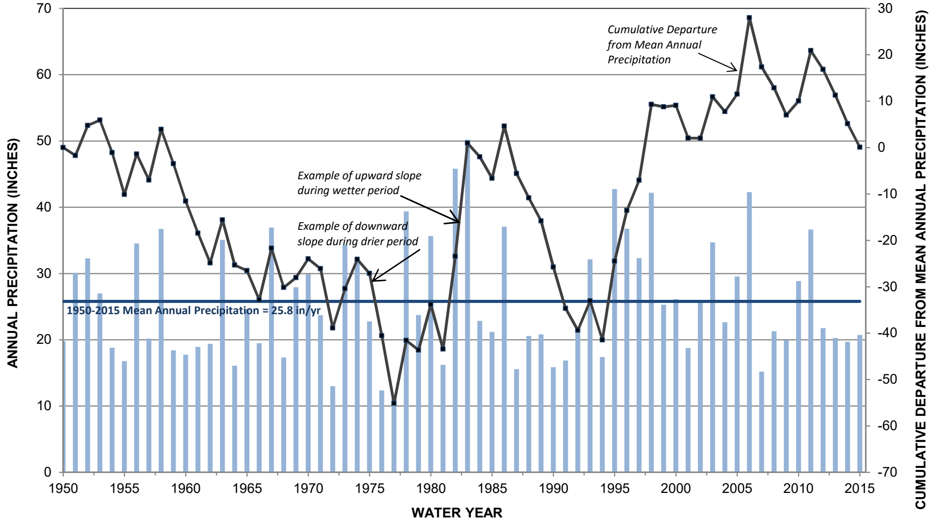
Figure 4-2 Napa State Hospital Water Year Precipitation and Cumulative Departure , Water Years 1950 - 2015
