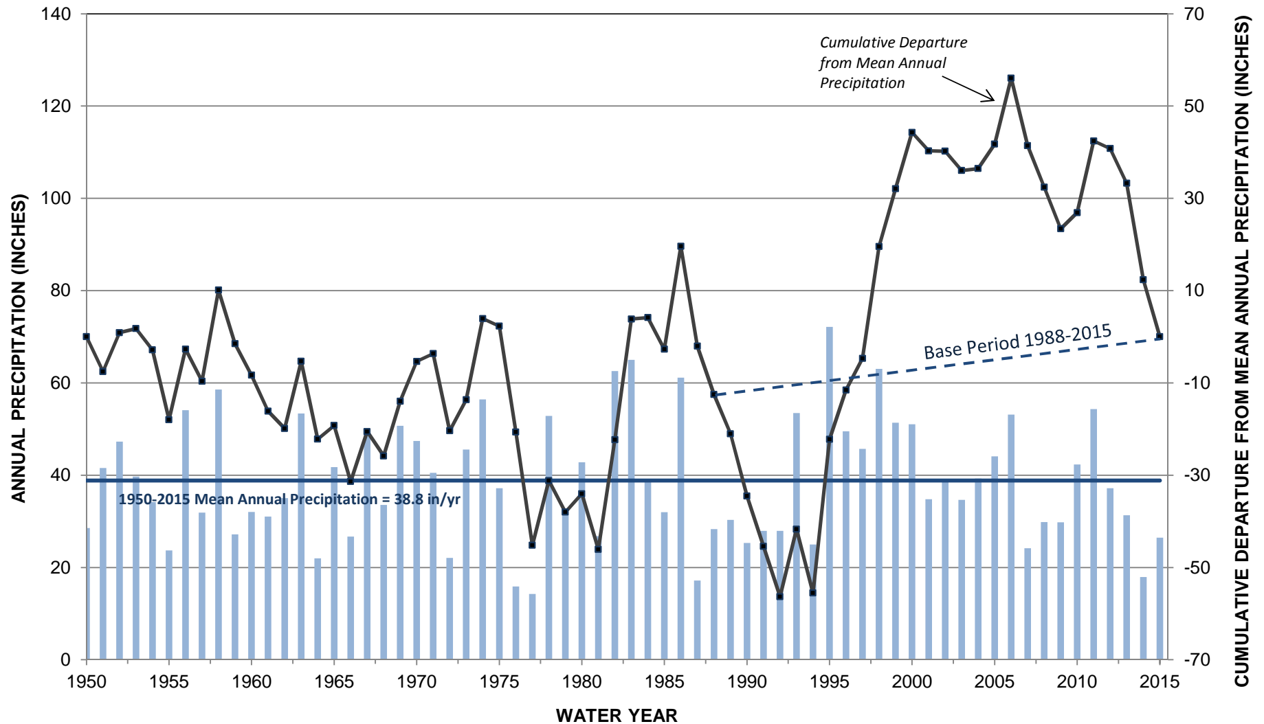
Figure 6-3 Calistoga Gage Water Year Precipitation (1950-2015) and Cumulative Departure
