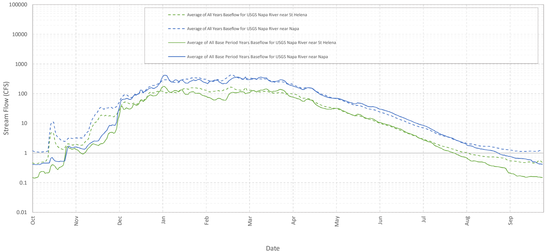
Figure 4-37 All Years Average Baseflow Analysis Results for the Napa River Near St Helena and Napa
