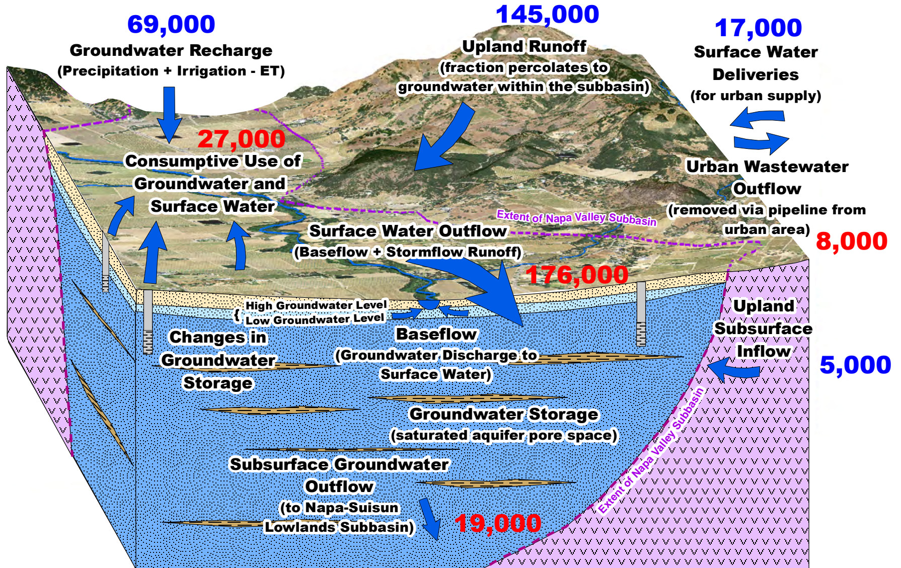
FIGURE 6-29 Schematic of Hydrogeologic Conceptual Model Components in the Napa Valley Subbasin with Average Annual Inflows and Outflows
