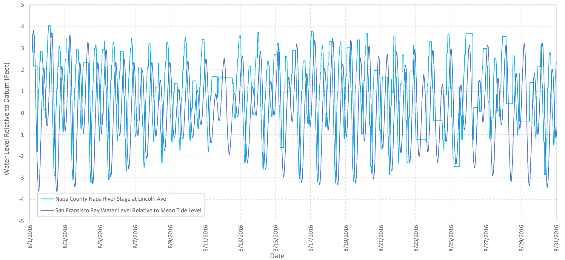
Figure 4-50 Example of Magnitude and Timing of Tidal and Lower Napa River Fluctuations
