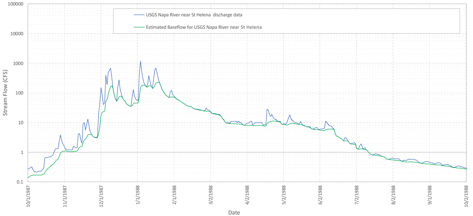
Figure 4-24 First Water Year Base Period Baseflow Analysis Results for the Napa River Near St Helena
