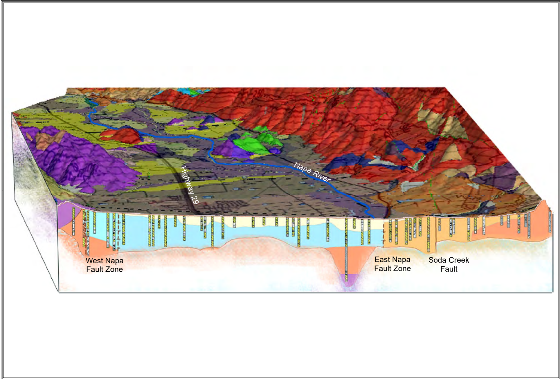
Figure 2-3 Three-Dimensional Visualization of the Geology in the Napa Valley Area
