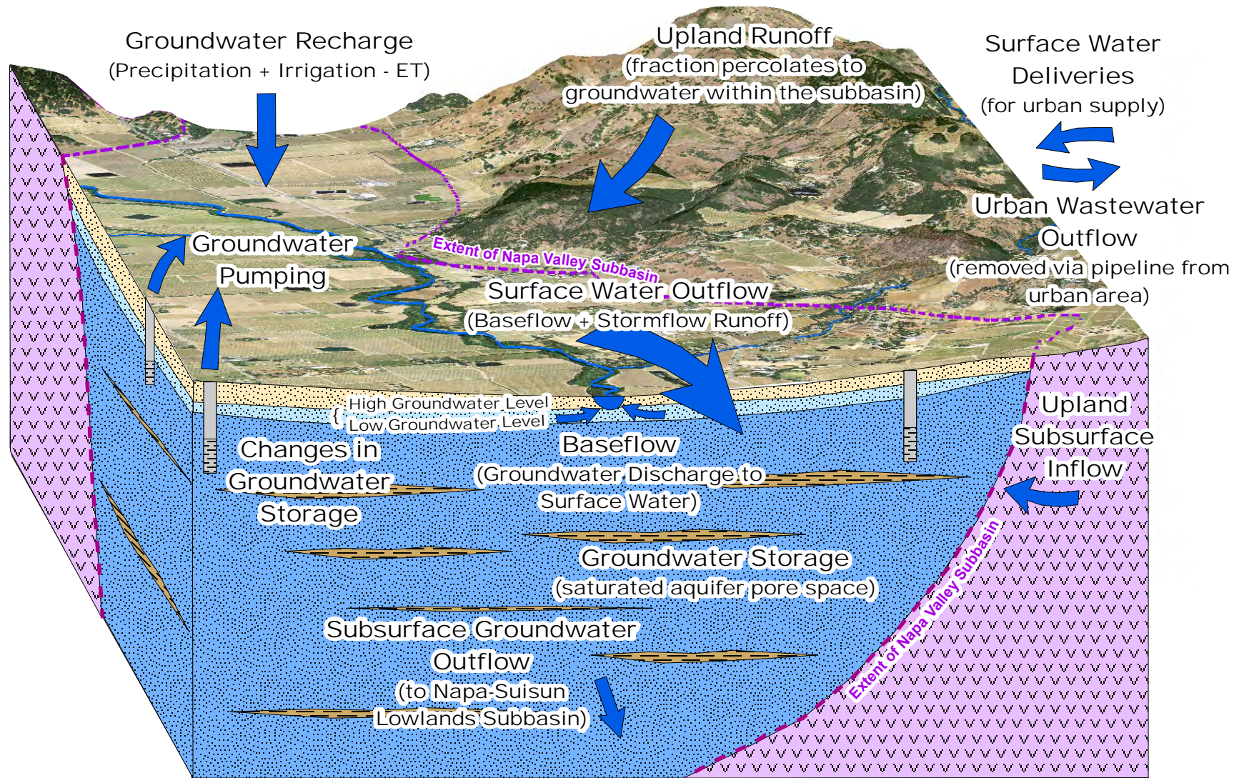
FIGURE 6-8 Schematic of Water Budget Components in the Napa Valley Subbasin
