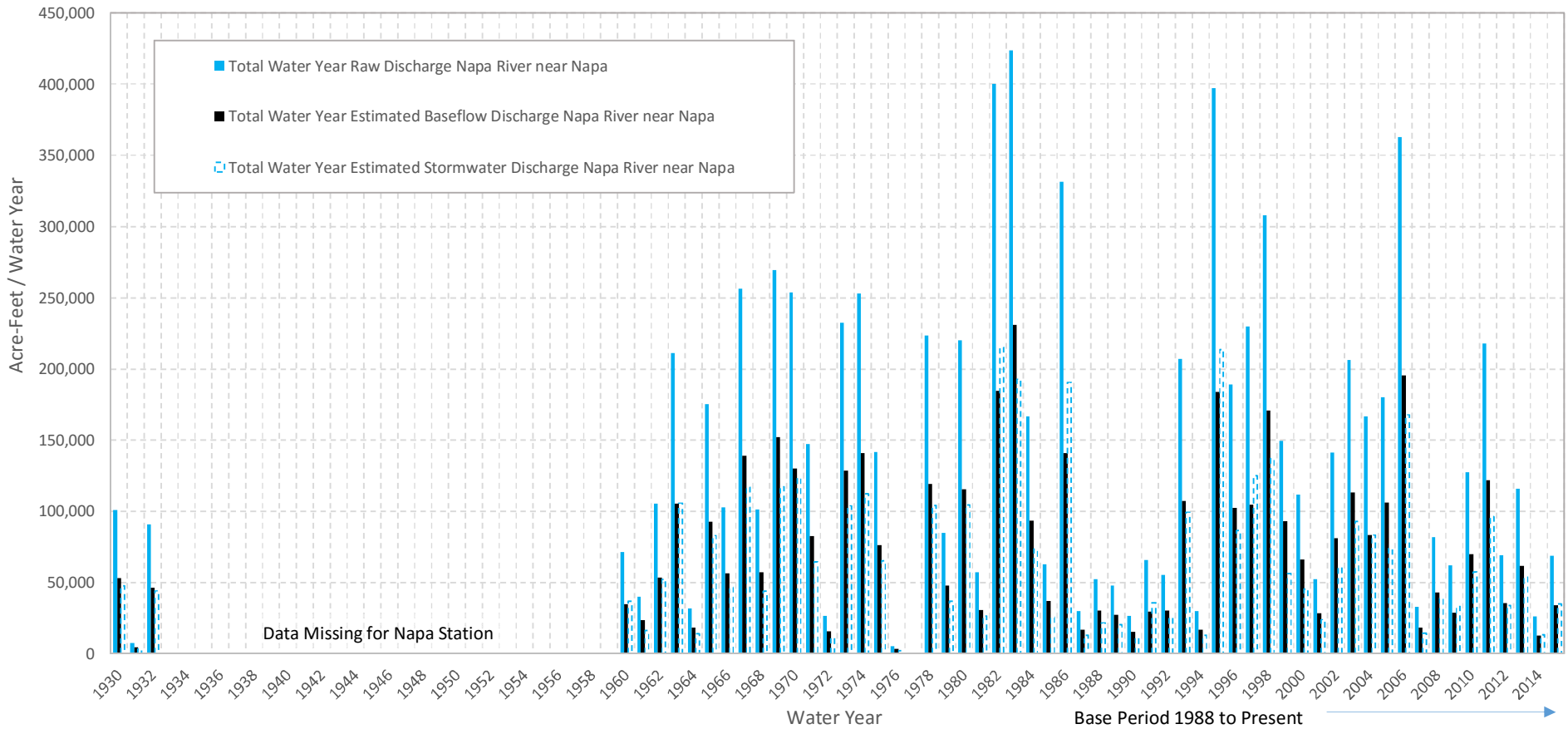
Figure 4-38 Total Napa River near Napa Discharge, Baseflow Discharge, and Stormwater Discharge
