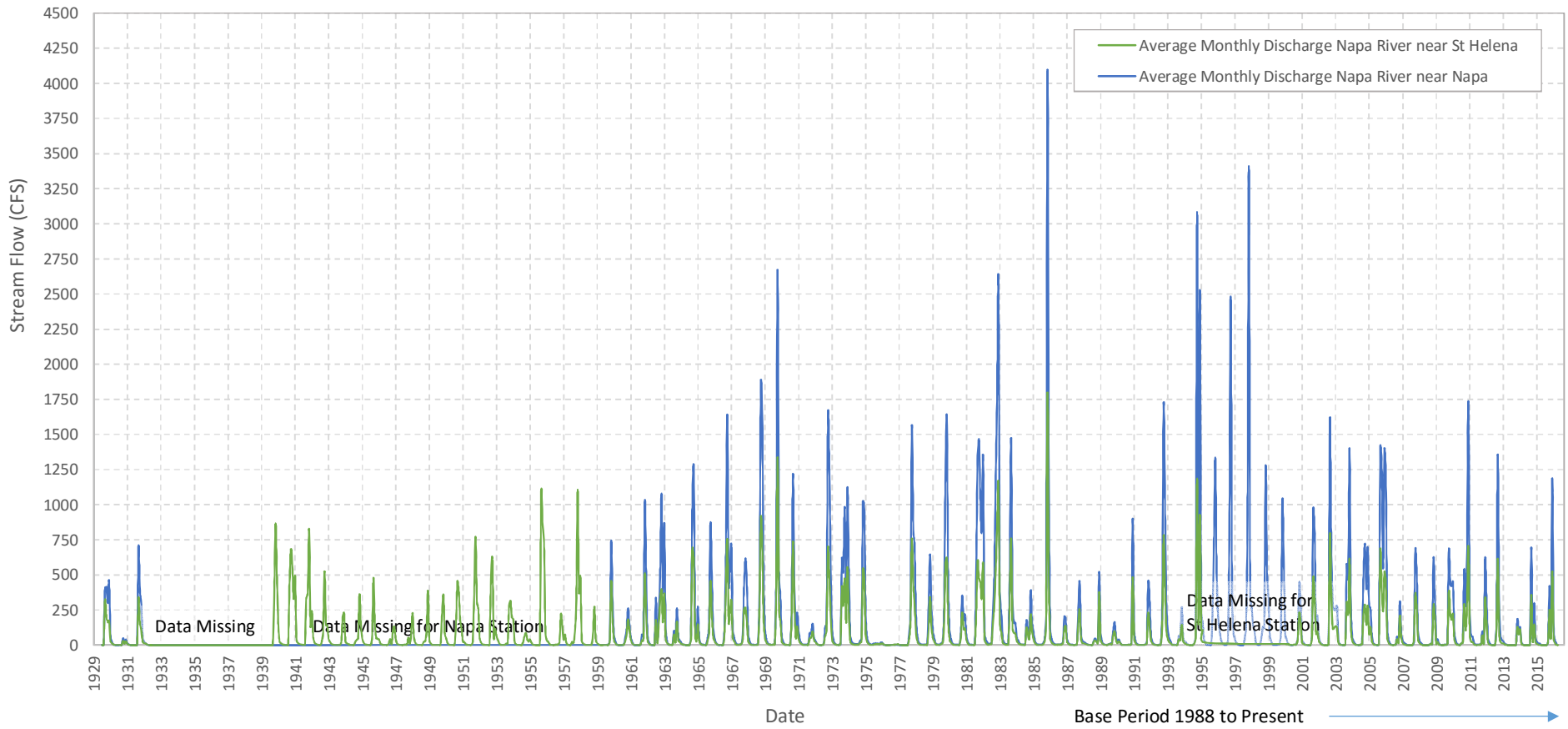
Figure 4-22 Historical Napa River Monthly Average Streamflow
