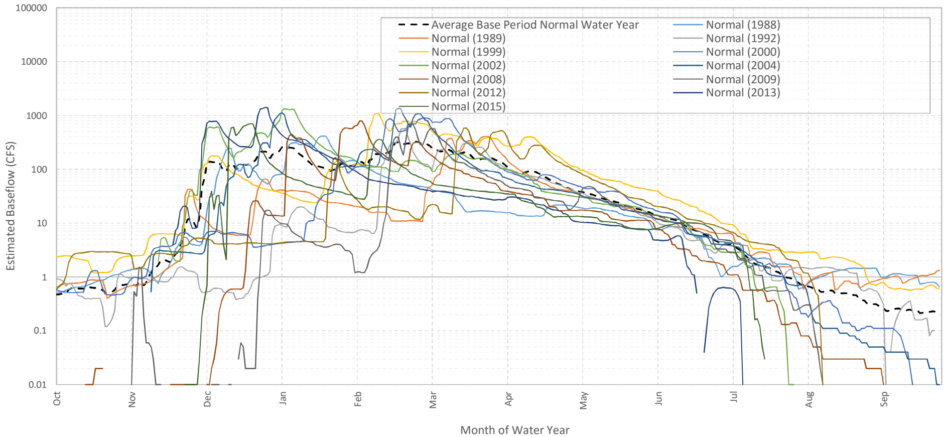
Figure 4-30 Base Period Baseflow Analyses Results for the Napa River Near Napa Normal Water Years
