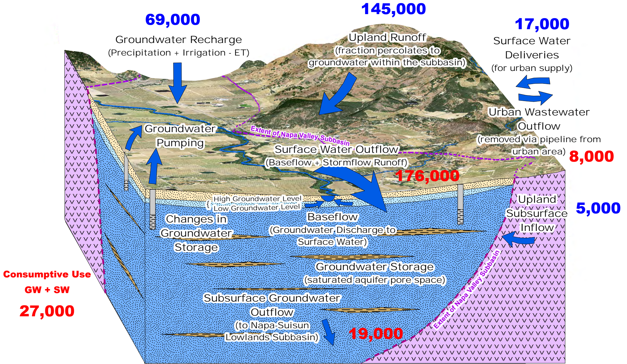
FIGURE 6-29 Schematic of Hydrogeologic Conceptual Model Components in the Napa Valley Subbasin with Average Annual Inflows and Outflows
