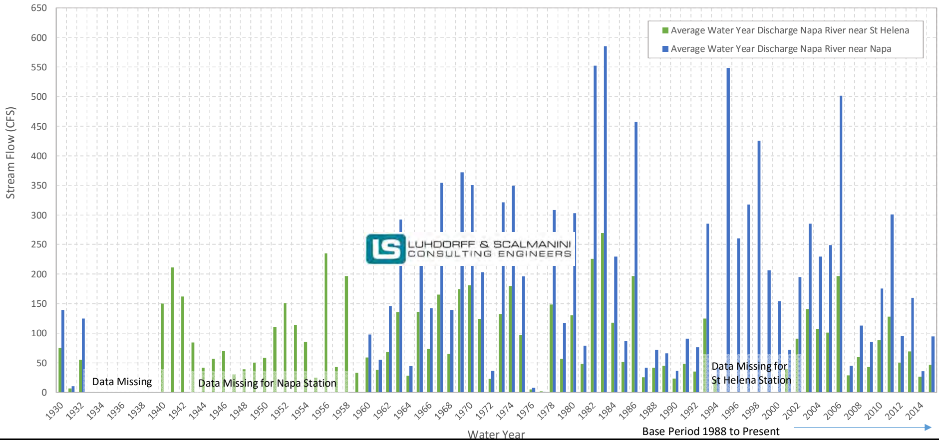
Figure 4-21 Historical Napa River Annual Average Streamflow by Water Year
