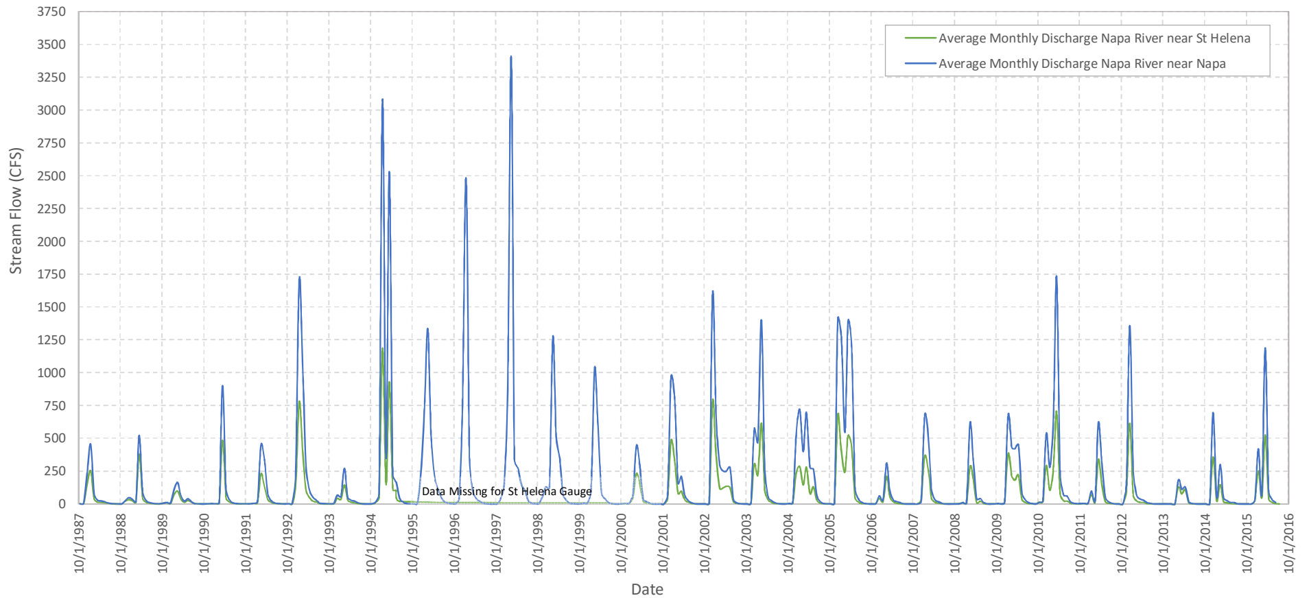
Figure 4-23 Base Period Napa River Monthly Average Streamflow Napa Valley Groundwater Sustainability A Basin Analysis Report for the Napa Valley Subbasin
