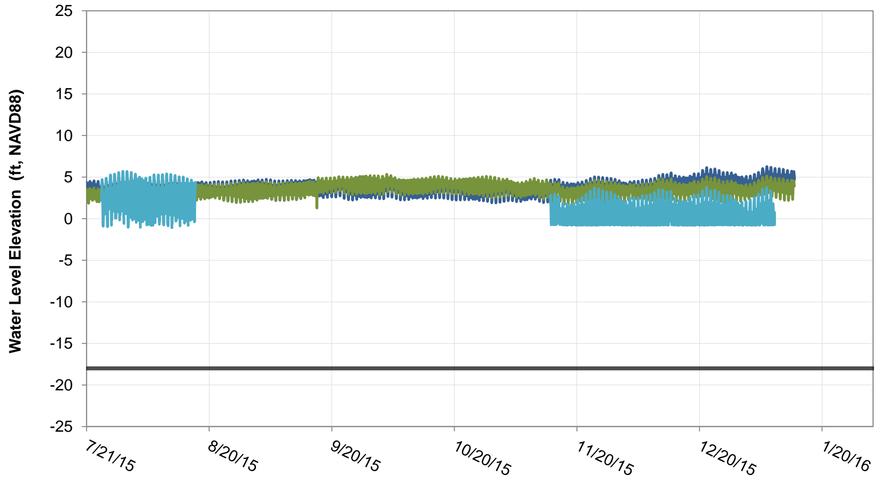
Figure 4-42 Surface Water-Groundwater Hydrograph Site 1: Napa River at First Street
