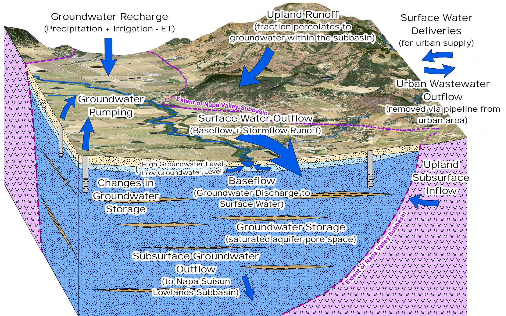
FIGURE 2-14 Schematic of Hydrogeologic Conceptual Model Components in the Napa Valley Subbasin
