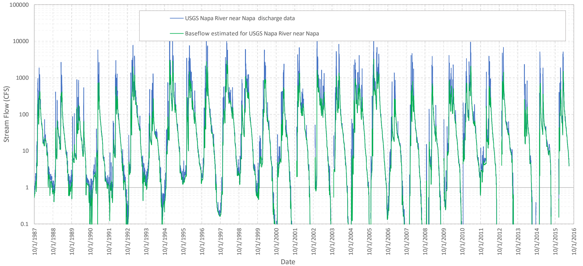
Figure 4-27 Base Period Baseflow Analysis Results for the Napa River Near Napa
