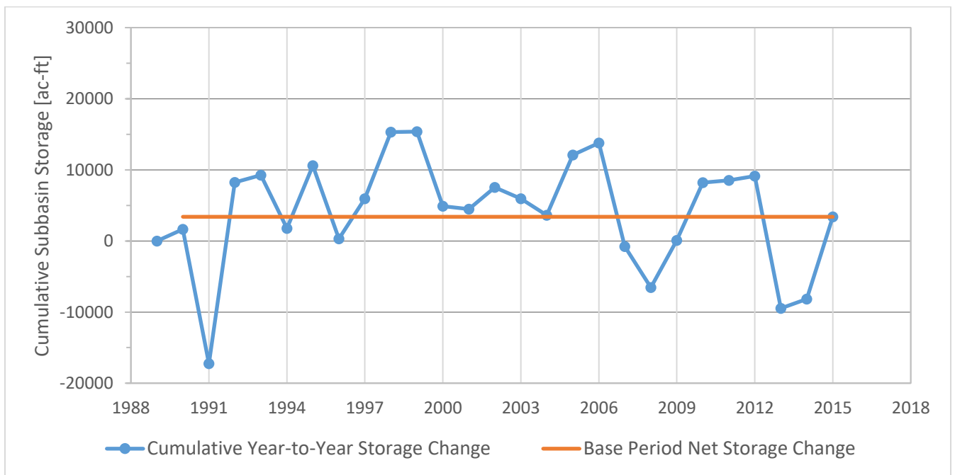
Figure 6-28b. Cumulative Groundwater Level Change in Storage
