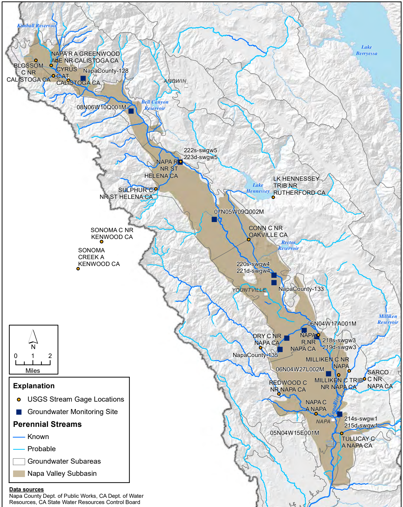
FIGURE 4-20 USGS Surface Water and DWR Groundwater Monitoring Sites
