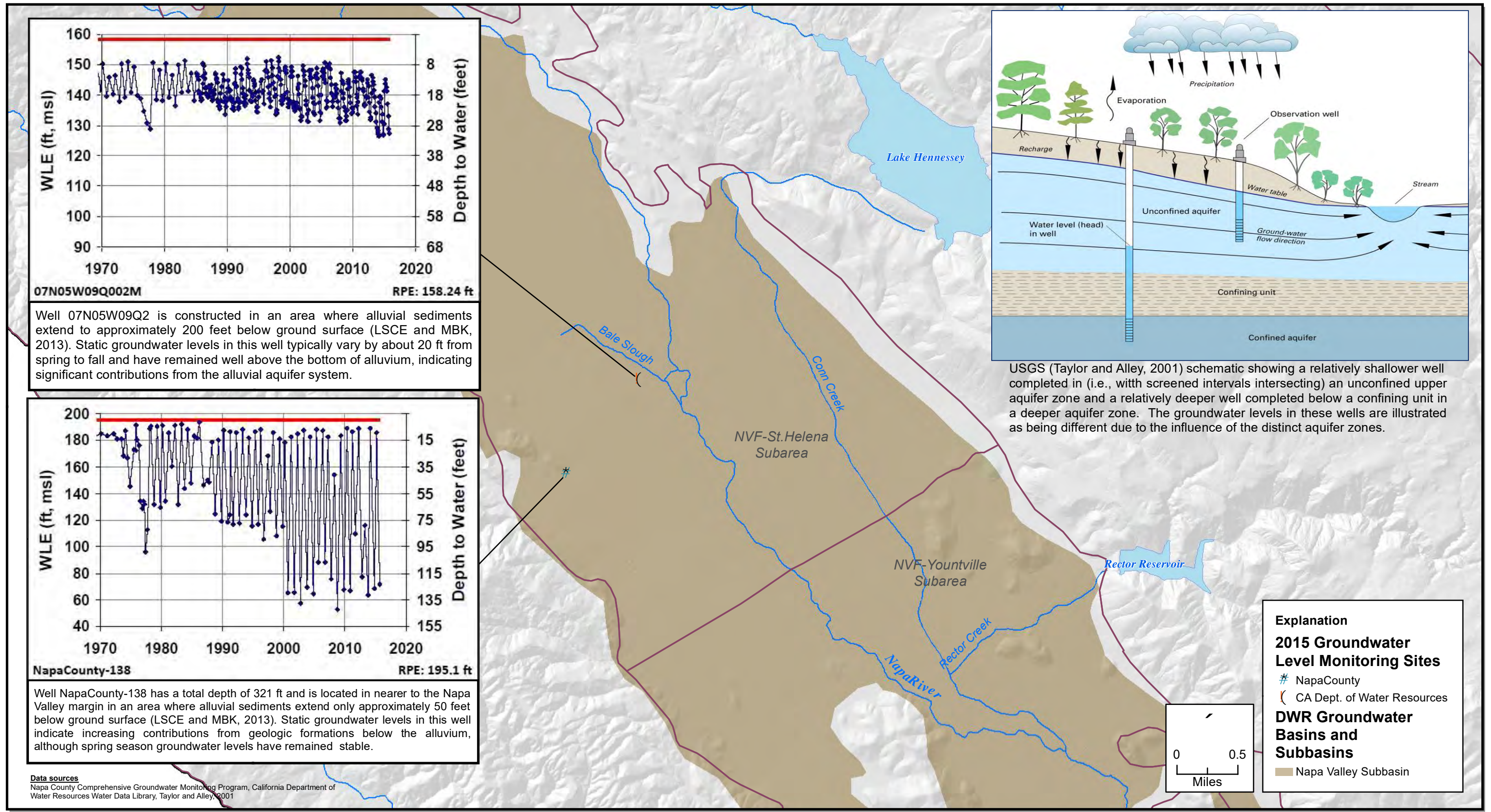
FIGURE 4-3a Southern St. Helena Subarea Aquifer Zone Schematic and Representative Hydrographs
