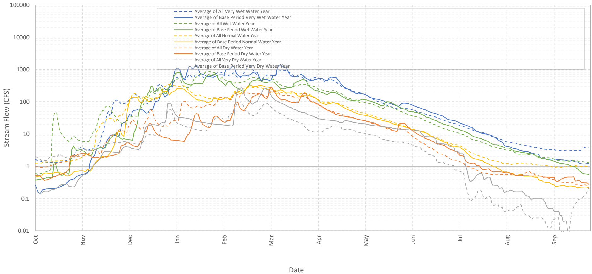
Figure 4-35 Average Water Year Type Baseflow Analysis Results for the Napa River Near Napa
